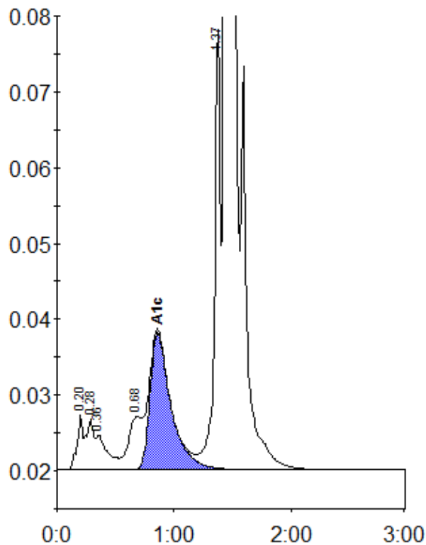
Peak table - ID: 10151453
